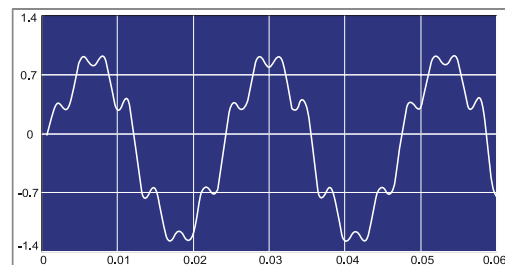
Harmonic Waveform
